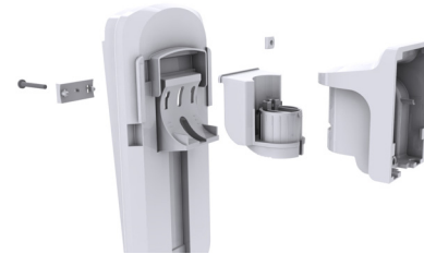
Figure 4: Exploded view of Swivel Bracket
