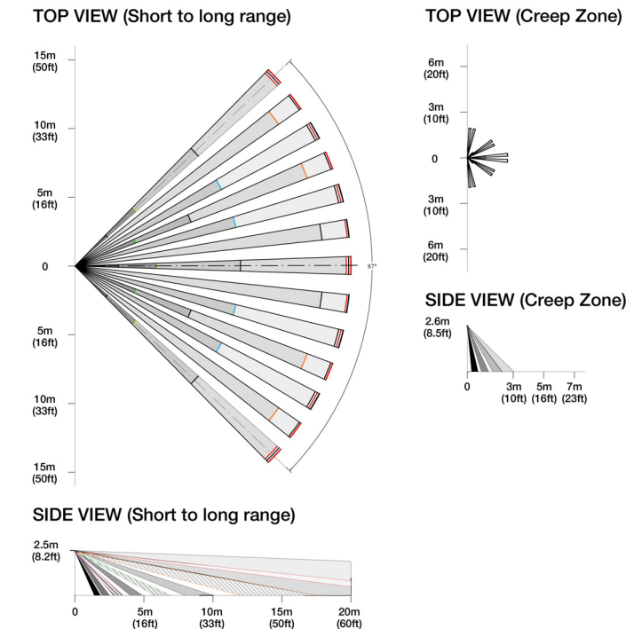
Figure 1: Beam Patterns
